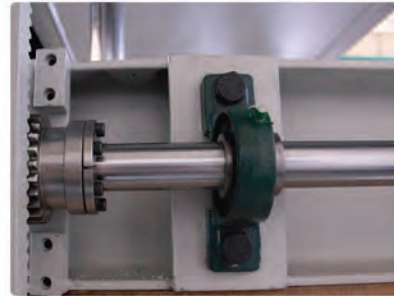
Homogen Pressure on Work Area with Mechanism of Toothed Rack
