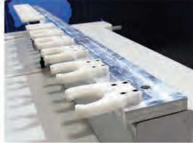
Tool Magazine (12 pieces)
